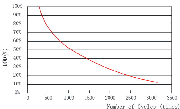
Cycle Service Life (35-40°C)
